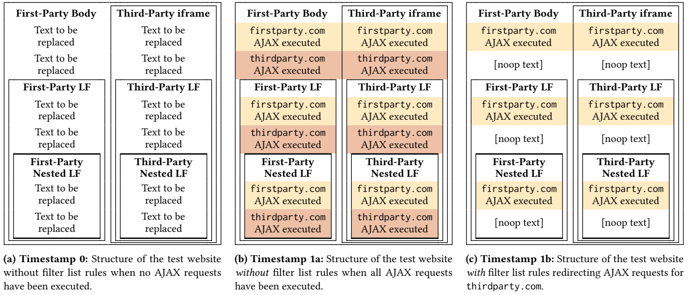
Figure 2: Structure of the test website for resource replacement before and after AJAX request execution ((a) and (b)), and the expected behavior of our test for RQ2 (c). Cells highlighted in yellow indicate successful AJAX requests from firstparty.com, and cells highlighted in red indicate successful AJAX requests from thirdparty.com.
