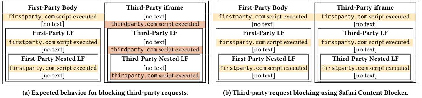
Figure 4: Structure of our test website for blocking requests. We find Safari Content Blocker’s interpretation of third-party requests differs from all other non-vulnerable tools, which match the expected behavior.
