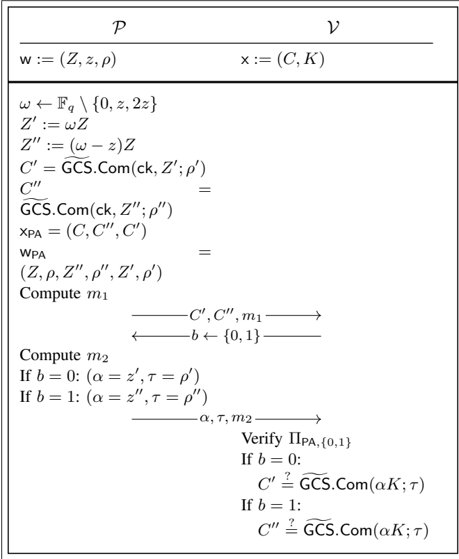
Figure 5: \Pi_{\text{SM}} : \mathcal{R}_{\text{SM}} \rightarrow \mathcal{R}_{\top} . In the above, m_1, m_2 denote the first and second prover message in an execution of \Pi_{\text{PA}, \{0,1\}} .
