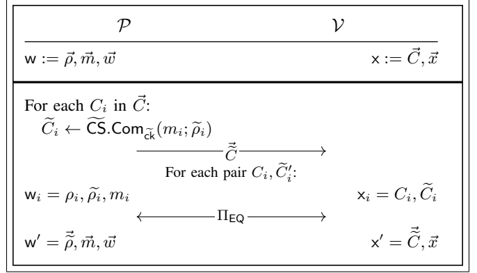
Figure 8: \Pi_{\mathcal{CS} \rightarrow \tilde{\mathcal{CS}}} : \mathcal{R}_{\mathcal{CS}, \mathcal{P}} \rightarrow \mathcal{R}_{\tilde{\mathcal{CS}}, \mathcal{P}} .
