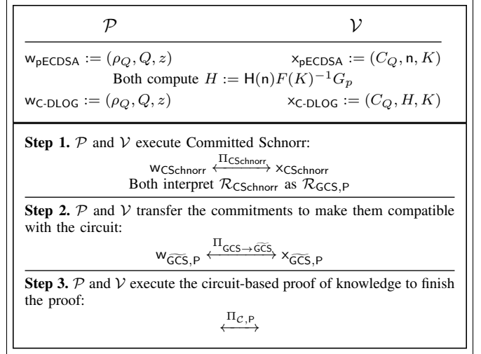
Figure 2: \Pi_{\text{Circ}} : \mathcal{R}_{\text{pECDSA}} \rightarrow \mathcal{R}_{\top} . The arrows indicate interactions between \mathcal{P} and \mathcal{V} .
