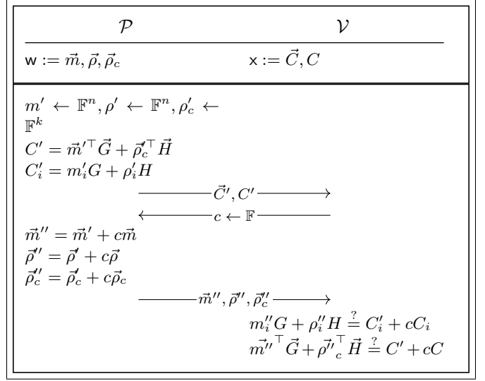
Figure 9: \Pi_{\text{PD}} : \mathcal{R}_{\text{EQ}} \rightarrow \mathcal{R}_{\text{T}} .
