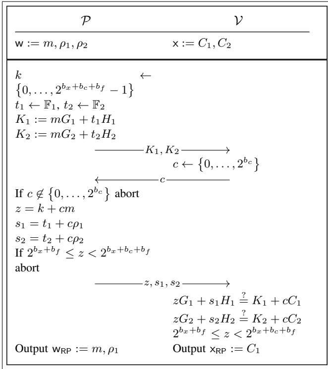
Figure 10: \Pi_{PD, \mathbb{G}_1, \mathbb{G}_2} : \mathcal{R}_{EQ, \mathbb{G}_1, \mathbb{G}_2} \rightarrow \mathcal{R}_{RP} .
