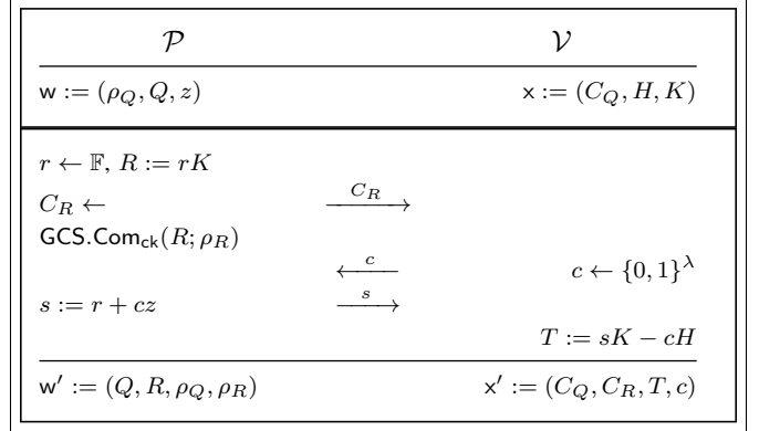
Figure 1: \Pi_{\text{CSchnorr}} : \mathcal{R}_{\text{C-DLOG}} \rightarrow \mathcal{R}_{\text{CSchnorr}} .
