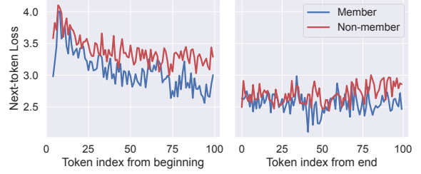
Figure 2: Average token losses at the beginning (left) and end (right) of sequences (Pythia-160M, Arxiv domain). Early tokens exhibit clearer differences between members and non-members, justifying our cut-off approach.
