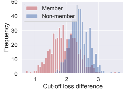
Figure 5: Distribution of loss differences after repeating inputs once ( f_{\text{Rep}}^1 ) (Pythia-160M, Arxiv domain). Non-members benefit significantly more from repetition, exhibiting larger loss reductions than members, clearly highlighting memorization differences.
